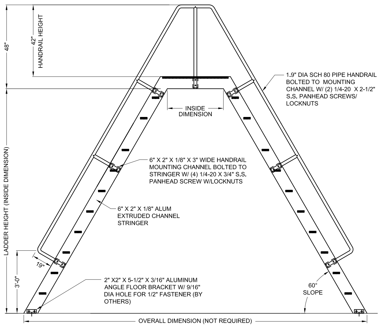
SIDE ELEVATION 3/8" = 1'-0"
