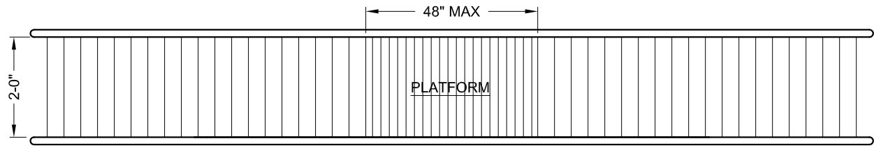
PLAN 3/8" = 1'-0"
