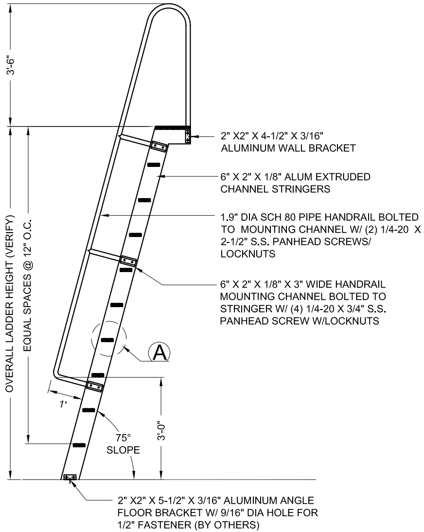
SIDE ELEVATION 3/8" = 1'-0"
