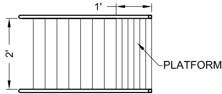
PLAN 3/8" = 1'-0"
