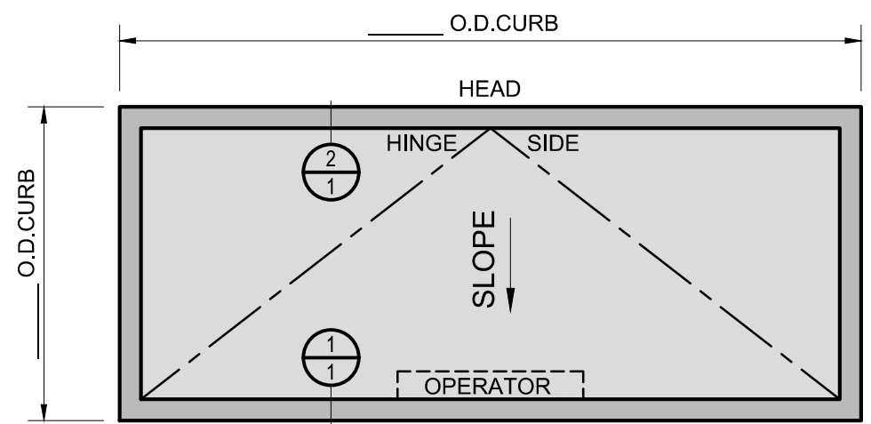
PLAN VIEW 3/4" = 1'
